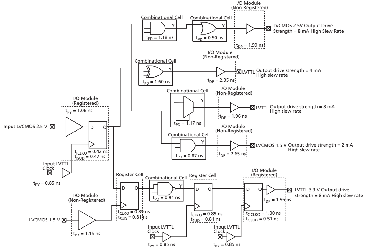
Figure 2-3 • Timing Model
